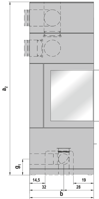
Front view and top view: SENDAI PRO 165
